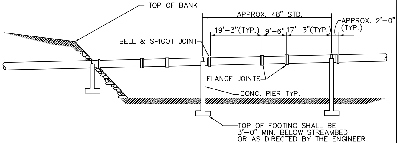
ELEVATED CROSSING – TYPE III (18" AND LARGER PIPE)
