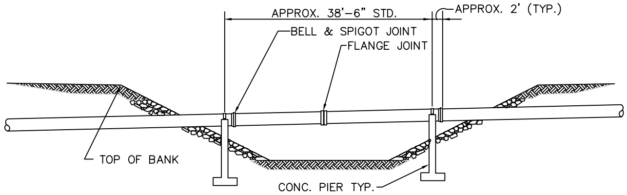
ELEVATED CROSSING – TYPE II
