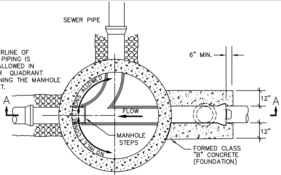
PLAN SECTION
