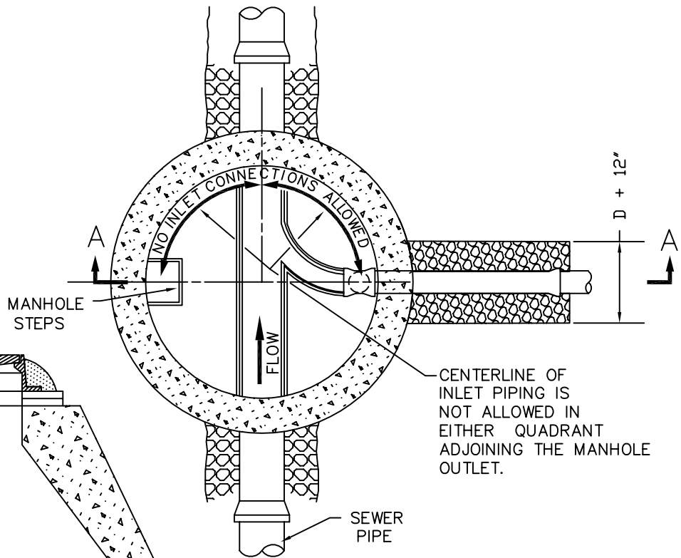
SECTIONAL PLAN
